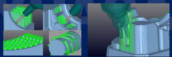
5-axis Conversion tool path
